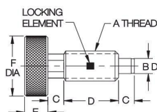
Standard Plunger
